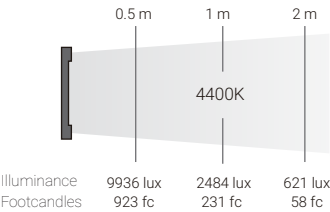
120° Beam Angle
